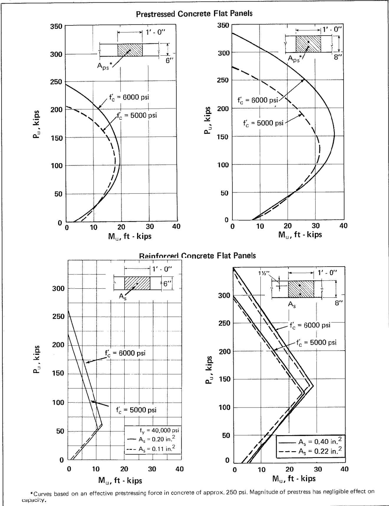
Fig. 3.6.2 Design (ultimate) capacity of prestressed and reinforced flat panels
