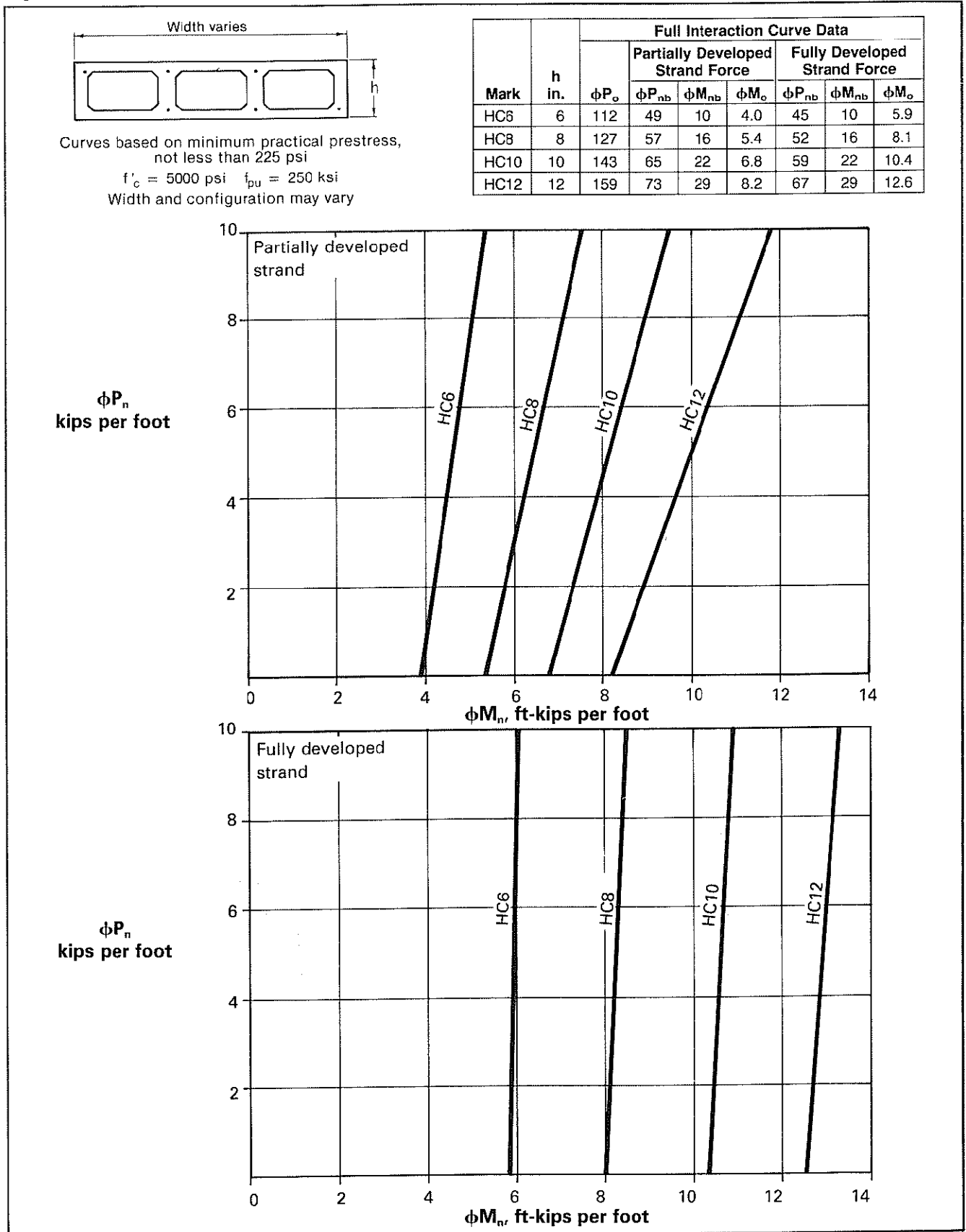
Fig. 2.6.4 Partial interaction curve for prestressed hollow-core wall panels
