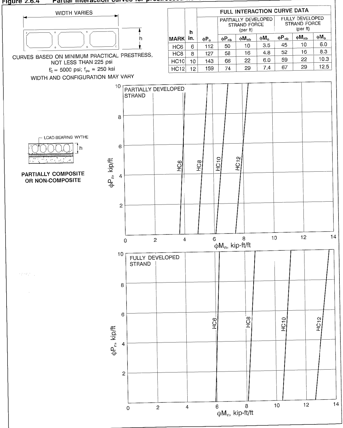
Figure 2.6.4 Partial interaction curves for prestressed hollow-core and sandwich wall panels
