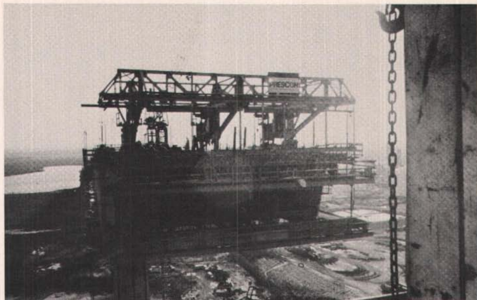
Fig. 10. Traveler set ready for concrete placement.
