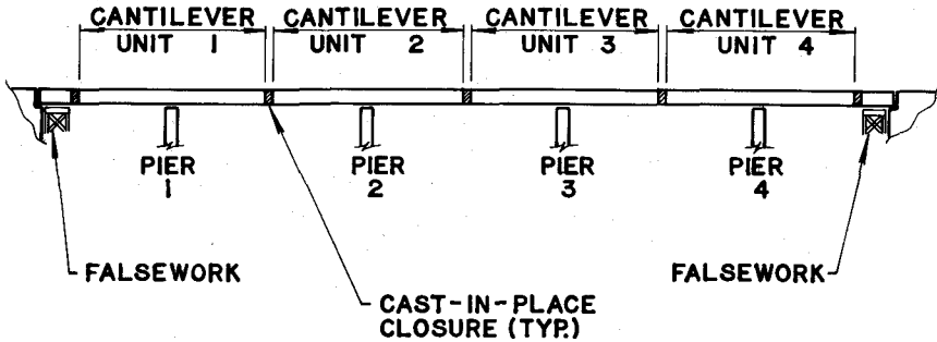
Fig. 3. Division of bridge into balanced cantilevers.
