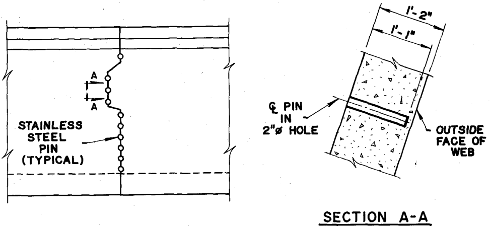
Fig. 25. Correction scheme for joints that contained non-hardened epoxy.
